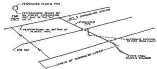
LAYOUT OF PERFORATED PIPE LATERALS FOR PRESSURE DISTRIBUTION BY MOUND
