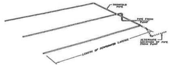
LAYOUT OF PERFORATED PIPE LATERALS FOR PRESSURE DISTRIBUTION BY MOUND
